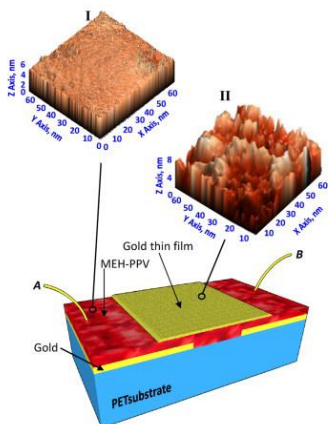
Structure of the fabricated humidity sensor.
